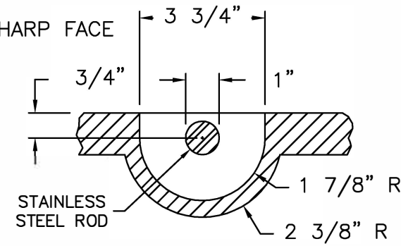
PICKBAR DETAIL
