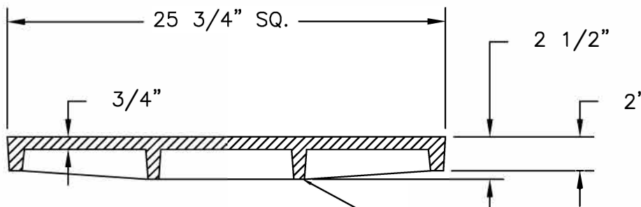
COVER SECTION
